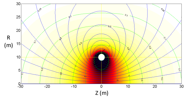
Figure 5. Flux lines and magnetic contours for a dipole torus. Here the current flows only at the toroid surface such that the magnetic field vanishingly small inside.
