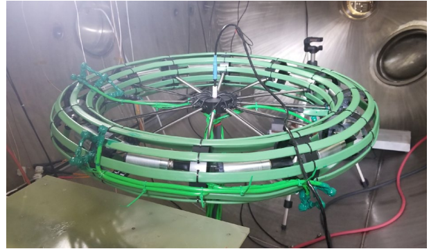
Figure 27. Magnetic field B_{00} calibration setup. High current cable leads can be seen on the vacuum tank floor. An array of 12 Faraday cups were positioned around the torus to collect the 600 eV protons from the ion beam.
