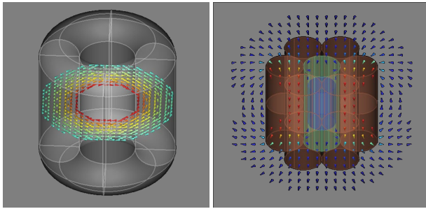
Figure 2. 2-D magnetic vector plots for (Left) ESA toroid at midplane, and (Right) 6-1 solenoids. The vectors are color coded red to blue indicating magnitude of the field. The plots range from the maximum field down to 5% of the maximum. The ESA toroid had no external fields larger than 1% of the maximum outside of the torus.
