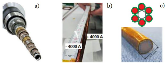
Figure 19. MgB 2 cables. From left: a) prototype power transmission cable made from MgB 2 tape (~3,000 A DC at 20 K, Diam ~ 30 mm); b) twisted-pair cable made from MgB 2 tape (~4,000 A DC at 4.2 K, Diam ~ 5 mm); c) top: prototype cable (consisting of six sub-cables) made from round MgB 2 wire (20,000 A DC at 24 K, Diam ~ 20 mm); bottom: one of the six sub-cables each made from 18 MgB 2 wires, of 1 mm diameter, helically wound around a copper core; All quoted critical currents are in self-field conditions (~1 T).
