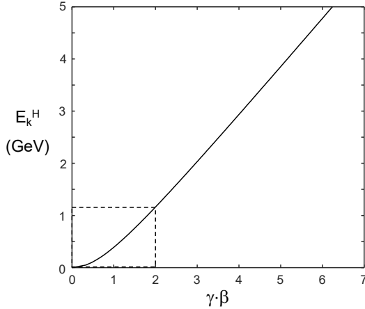
Figure 30. Relativistic proton energy as a function \gamma\beta .
