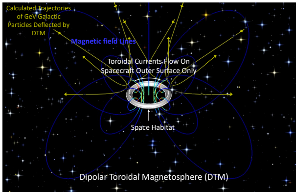
Figure 4. Dipolar magnetospheric shielding provided by toroidal currents I.e. The HTSC magnet (sliver colored shell) is placed external to the toroidally shaped space habitat. The magnet would fully surround the habitat to assure cancelation of all magnetic field inside the habitat.
