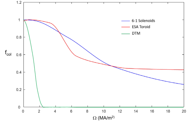
Figure 13. Fraction of 500 MeV protons reaching the habitat of the various concepts as a function of the efficiency parameter \Omega .
