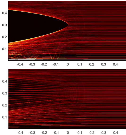
Figure 32. The figures above showing the difference in particle trajectory for a single large current bundle (top) as compared with a 15 \times 15 grid with the same total current (bottom). Proper coil concentration and current distribution can help protect from and redirect GCR away from coils.
